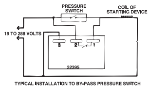
Low pressure switch bypass application.
